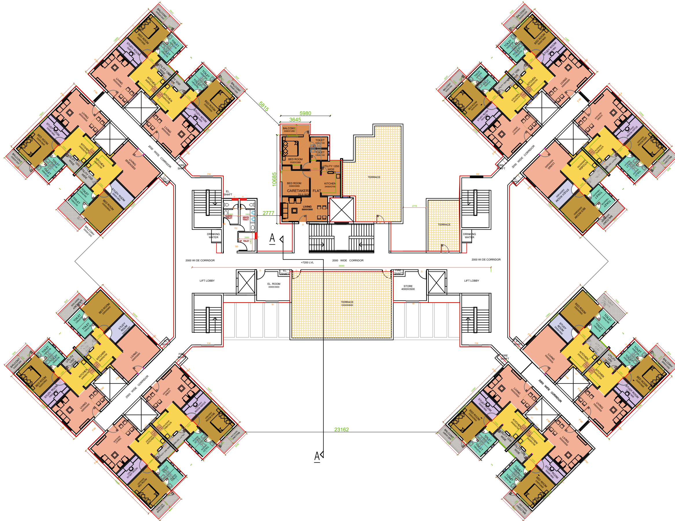
SECOND FLOOR PLAN 1861 SQM
